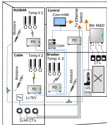
Switchgear Cell with monitoring Details
