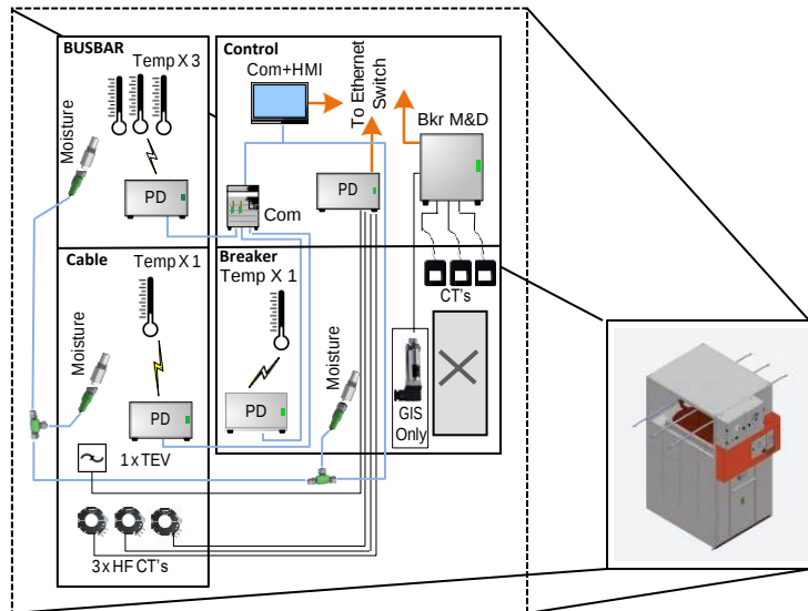
Switchgear Cell with monitoring Details
